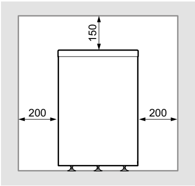
Minimum clearances
