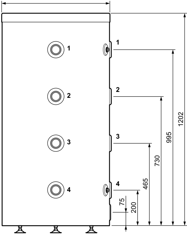
200 litre buffer vessel dimensions and connection dimensions
